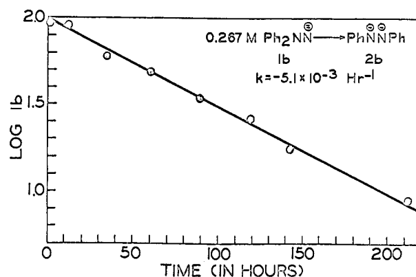
Figure 3. Typical plot of the logarithm of concentration of 1b in moles/liter vs. time. Methyl lithium:1 ratio in this experiment was 10.4:1. (At lower \text{CH}_3\text{Li} ratios deprotonation is rate limiting in early stages, and the first few points deviate somewhat from the linear relationship shown.)
