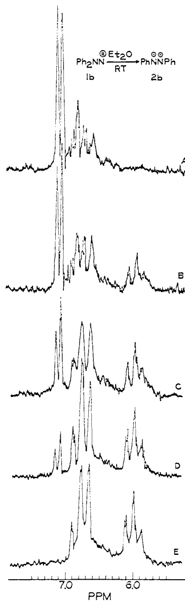
Figure 2. Nmr spectrum in the aryl region for the dianion 1b rearranging to 2b . Initial concentrations were 0.267 M 1 and 10.4 equiv of methyllithium in diethyl ether at 25°. Times (hr): A, 2; B, 32; C, 60; D, 143; E, >250.
